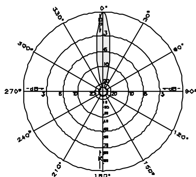
Diagrama Horizontal
