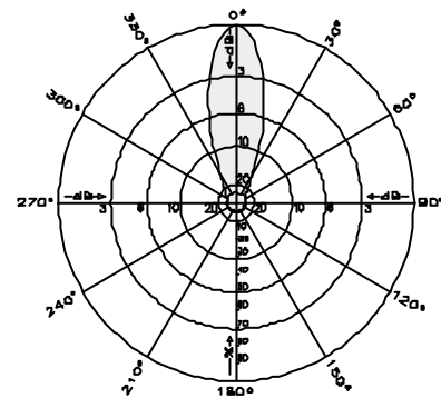
Diagrama Vertical
