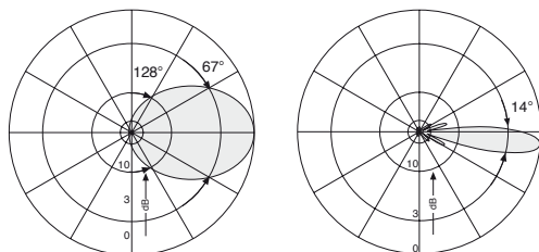
Diagrama Horizontal
