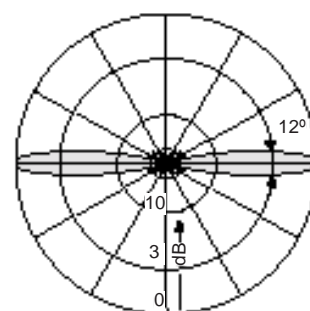
Diagrama Vertical
